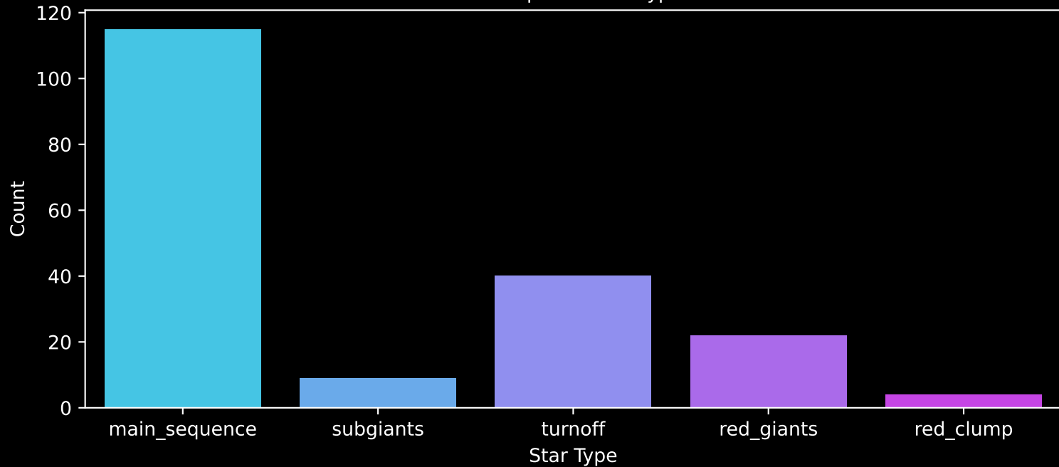
APOGEE DR17 Field: [163+81_MGA] Count plot of Star Type
